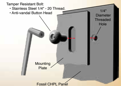
② Attaching Panel to Hardware
