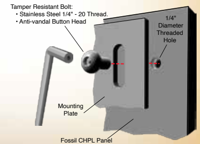
2 Attaching Panel to Hardware
