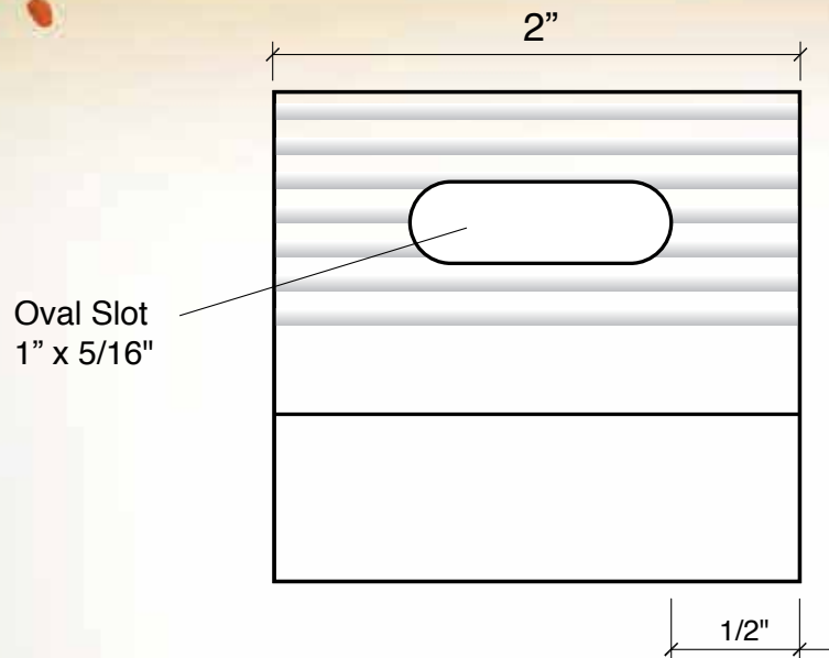
1 Front View - "Z" Bracket
