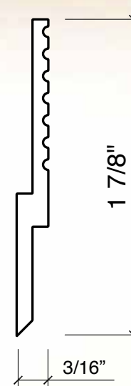
2 Side View - "Z" Bracket
