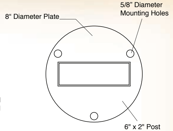
2 8" Diameter Base Plate (6x2 Post)
