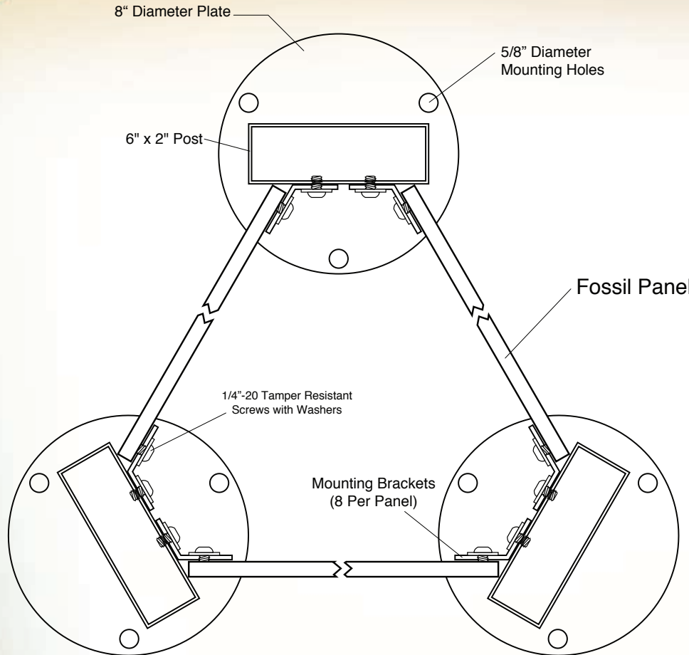
Triangular Kiosk - Top View
