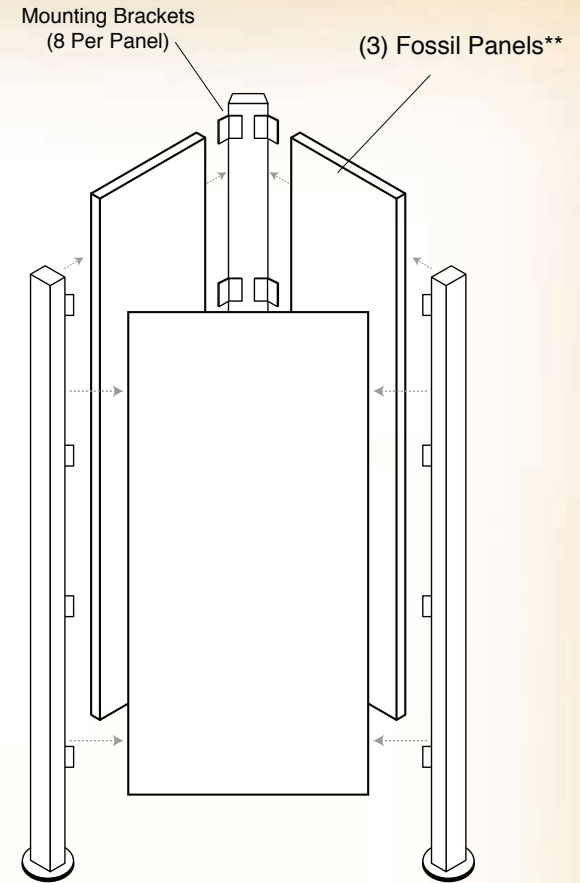
Multiple Post Assembly
