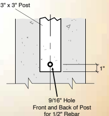
② Underground Portion of Post
