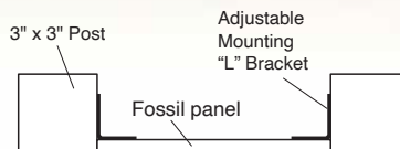
Even Mount
