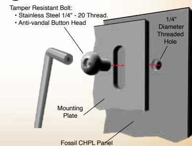
③ Attaching Panel to Hardware
