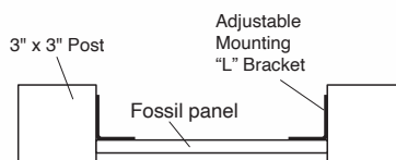
Recessed Mount
