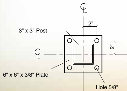
① Base Plate (3x3 Post)
